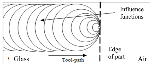
Figure 3. The use of tool-lift to reduce spot-size in the vicinity of an edge
